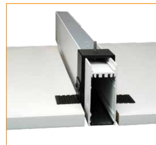
trimless mounting kit ☑ minimum 39mm x profile length ref: XLTRMO € 6,50
