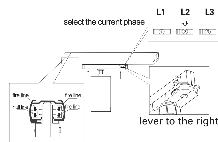
Install track adapter in the direction indicated in above picture
